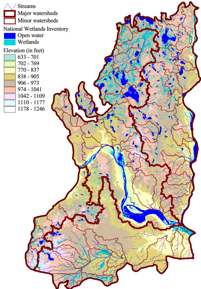
Elevation, Watersheds, and Surface Hydrology
